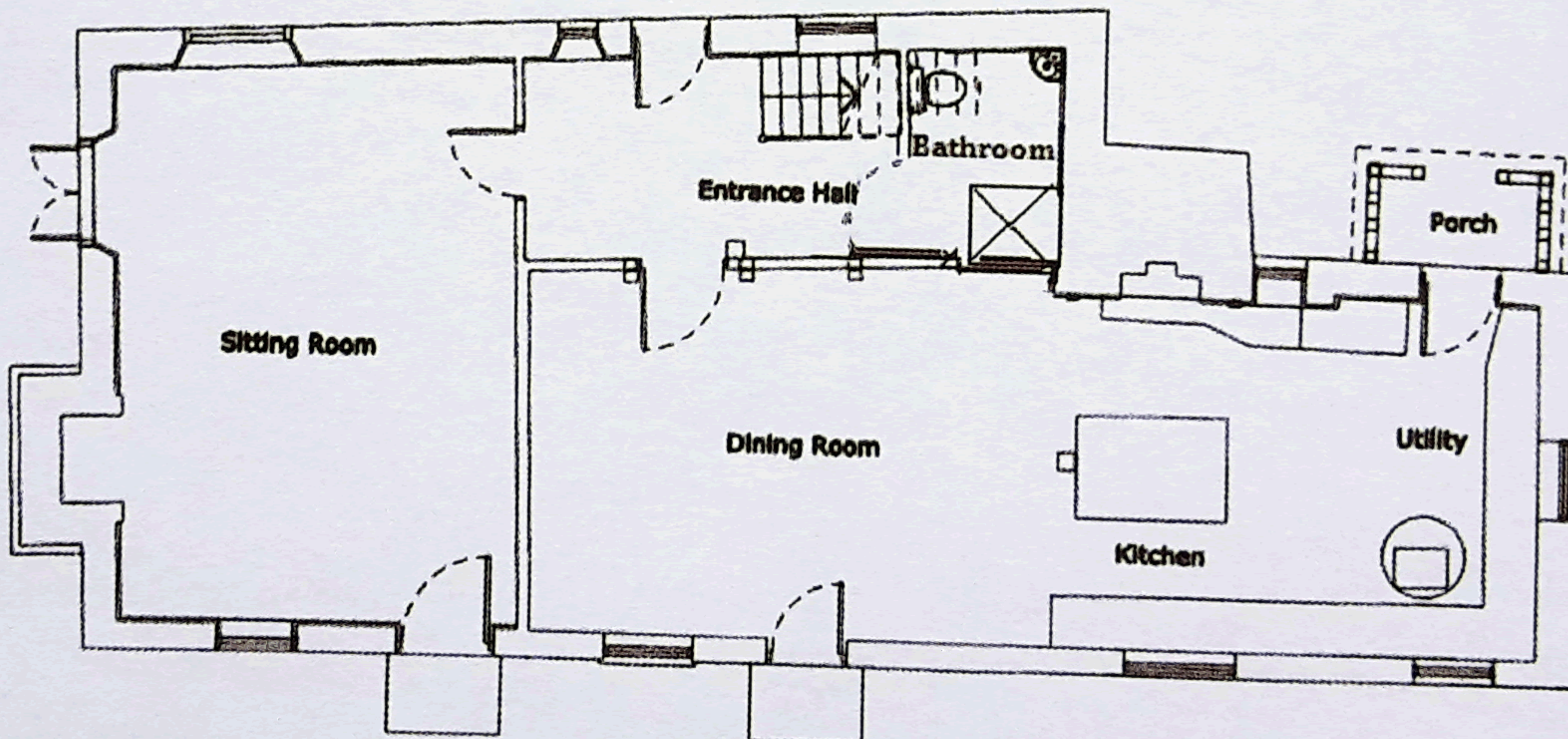
LITTLE CANWOOD HOUSE - GROUND FLOOR PLAN
